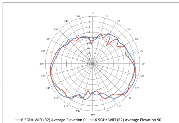
6.5GHz Wi-Fi antennas patterns (vertical)
