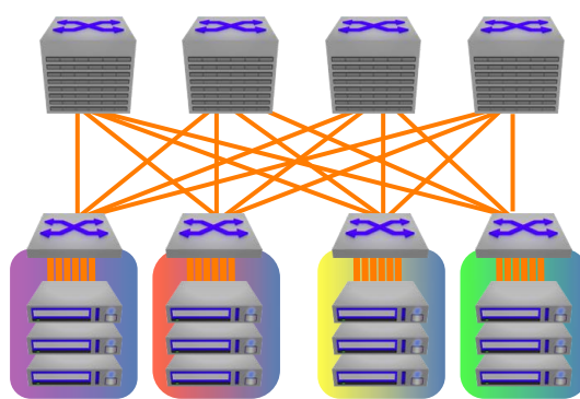
Arista Modular System Leaf-Spine Designs Scale to 55,296 25/50GbE ports at 3:1 subscription in a 16-way ECMP Design
